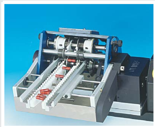
CS40 FEEDER for TP6/PR-F (Cod. 51.0400)
